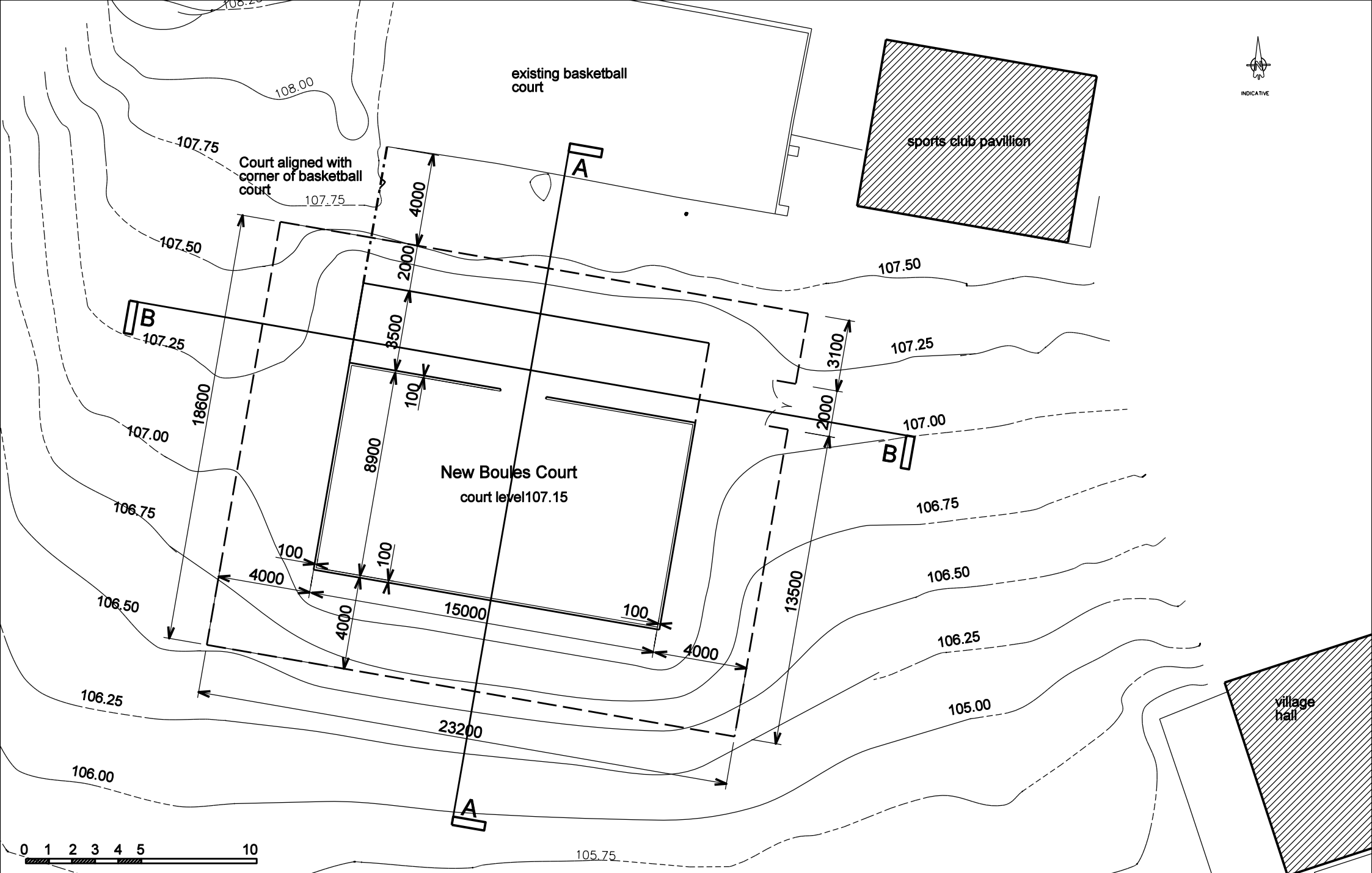
West Meon Boules Court Dimensions and Setting Out
